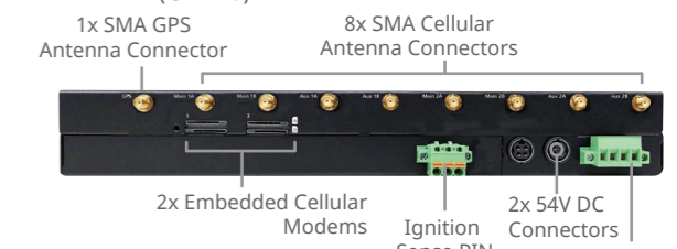
Back: 1x SMA GPS Antenna Connector, 8x SMA Cellular Antenna Connectors
