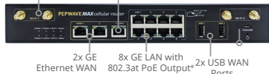
RP-SMA Wi-Fi WAN Antenna Connectors, 1x GE Ethernet WAN/ LAN*, RP-SMA Wi-Fi AP Antenna Connectors
