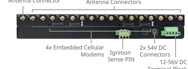
HD4 MBX (CAT-18): 1x QMA GPS Antenna Connector, 16x QMA Cellular Antenna Connectors
